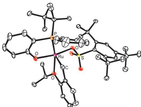
Figure 3. Crystal structure of complex 2e (ORTEP plot, 20% probability ellipsoids).
