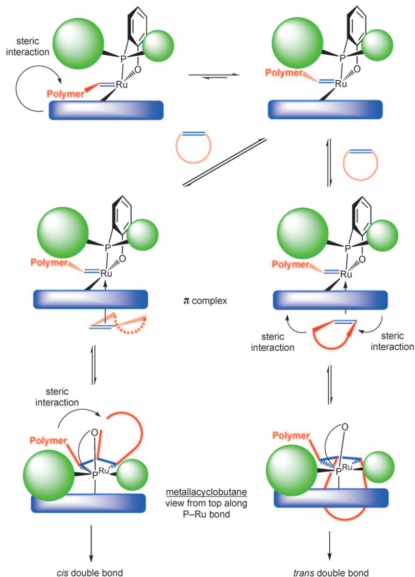
Scheme 2. Mechanistic explanation of the stereochemistry of double bonds.
