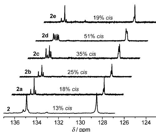
Figure 1. ^{13}\text{C} NMR spectra showing the alternating copolymerization of norbornene and cyclooctene in \text{CH}_2\text{Cl}_2 with increasing cis content from bottom to top using asymmetric catalysts 2–2d prepared in situ and low selective catalyst 2e . (See ^1\text{H} NMR spectra in Figures S8 and S14 in the Supporting Information.)
