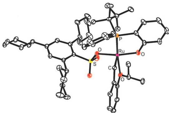
Figure 2. Crystal structure of complex 2d (ORTEP plot, 20% probability ellipsoids). Crystal structures for complexes 2a and 2f are given in the Supporting Information.
