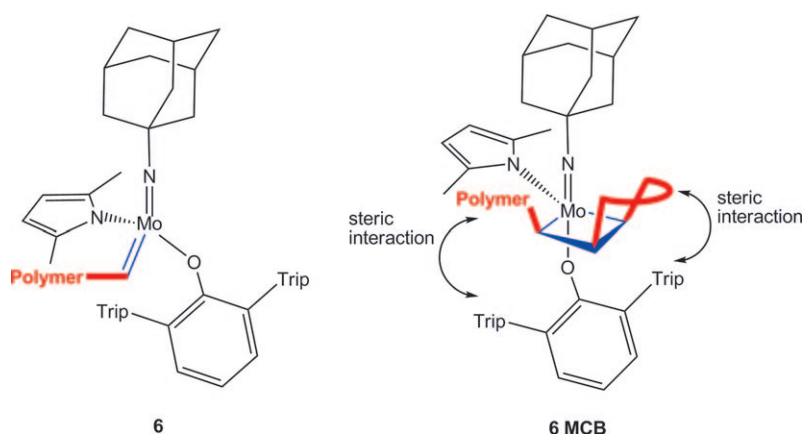
Scheme 3. Stereogenic-at-metal molybdenum complex 6 published by Schrock and Hoveyda for the Z -selective polymerization of norbornene derivatives and proposed metallacyclobutane structure 6 MCB with all- cis substituents.
